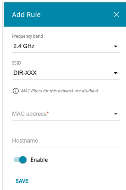
Figure 115. The window for adding a rule for the MAC filter.
