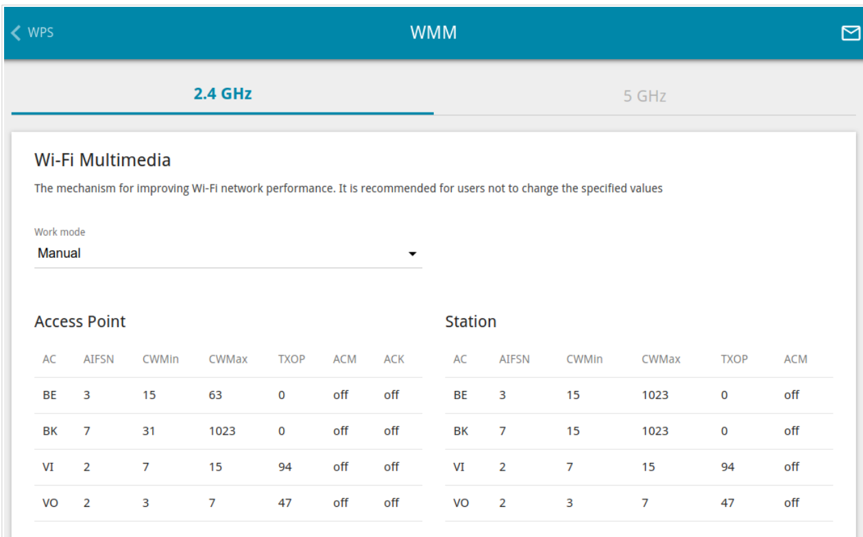
Figure 108. The page for configuring the WMM function.
