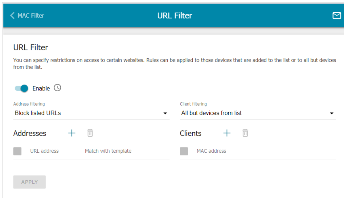
Figure 143. The Firewall / URL Filter page.
