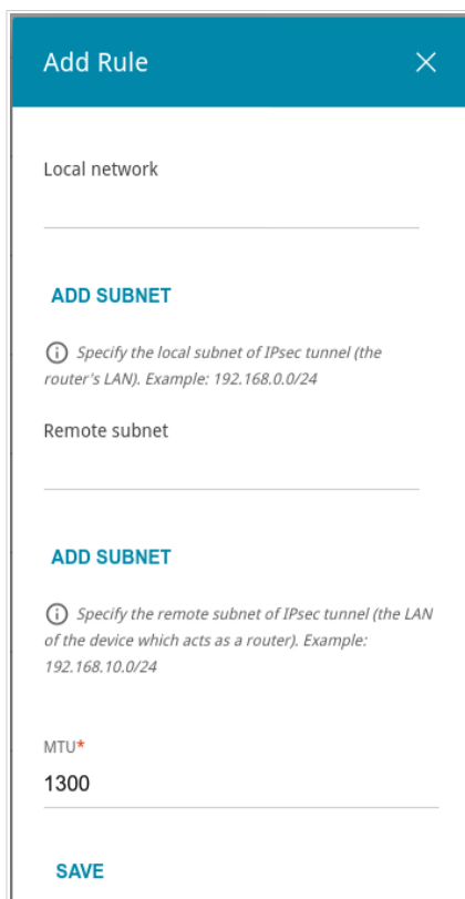
Figure 135. The page for adding an IPsec tunnel. The window for adding a tunneled network.
