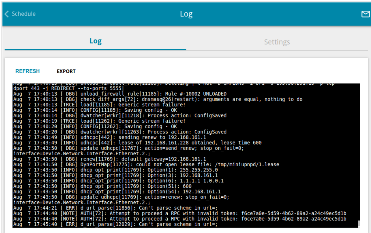
Figure 153. The System / Log page. The Log tab.
