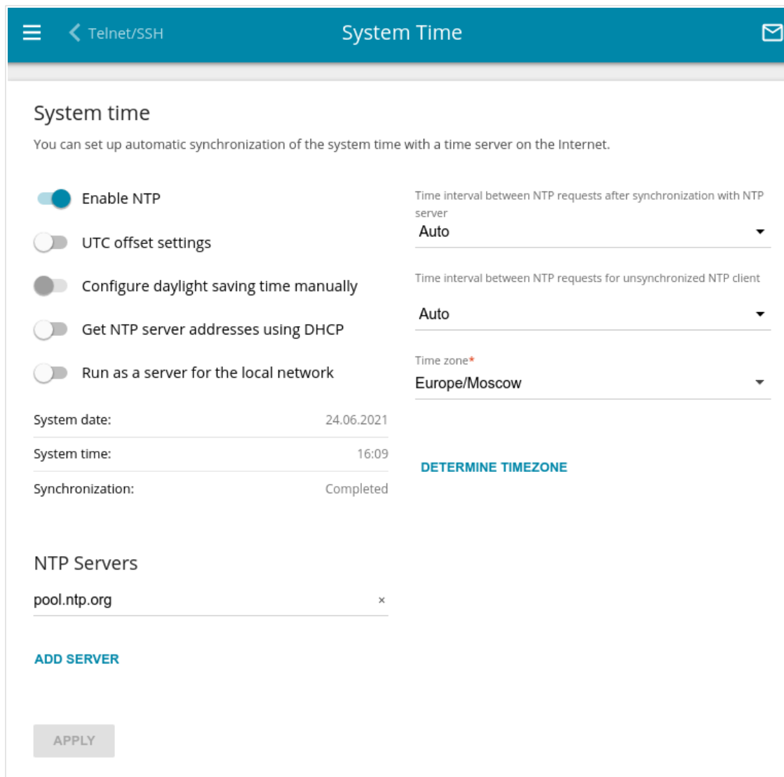
Figure 159. The System / System Time page.
