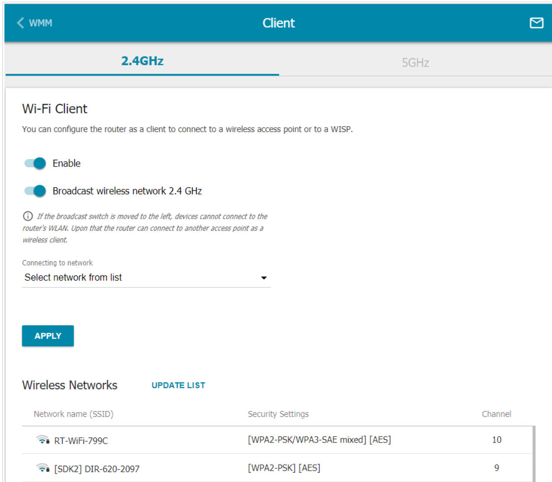
Figure 110. The page for configuring the client mode.
