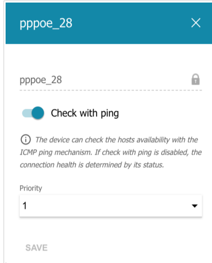
Figure 99. The window for changing the priority of a connection.
