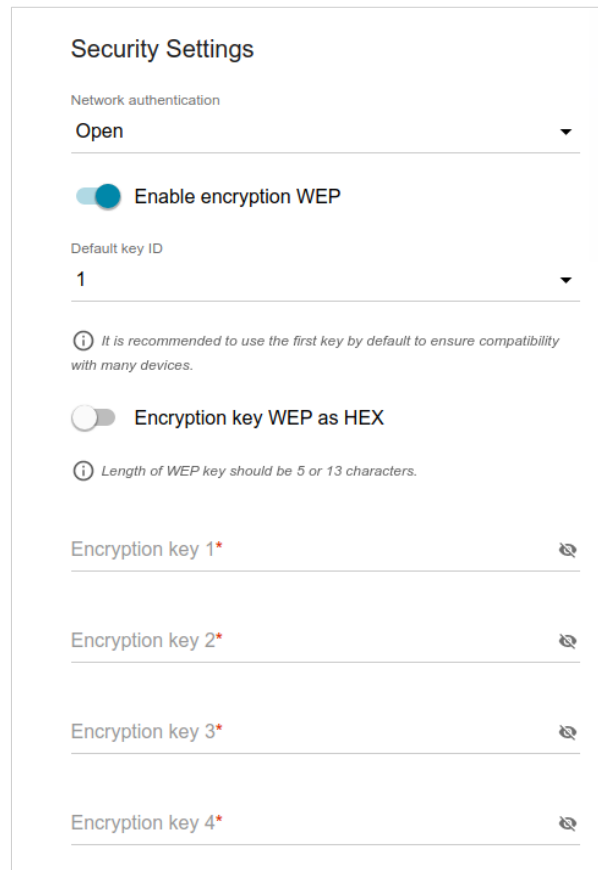
Figure 112. The Open value is selected from the Network authentication drop-down list.
