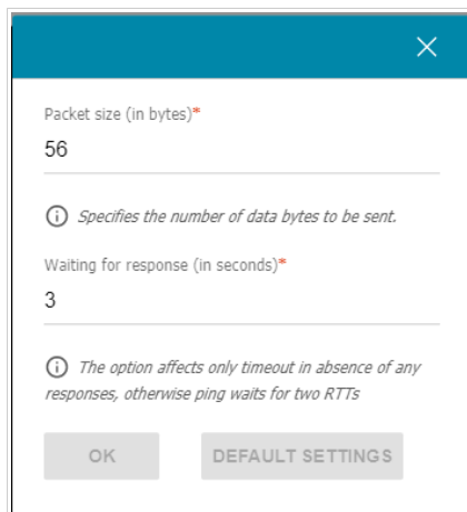
Figure 184. The System / Ping page. The additional settings window.
