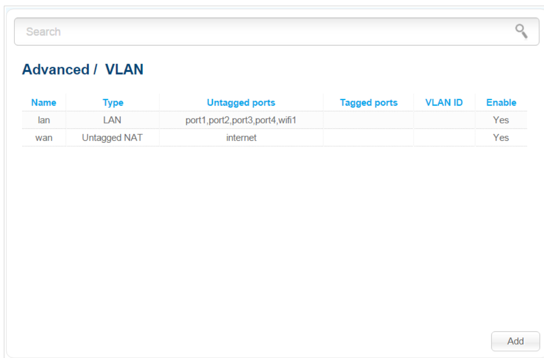
Figure 106. The Advanced / VLAN page.
