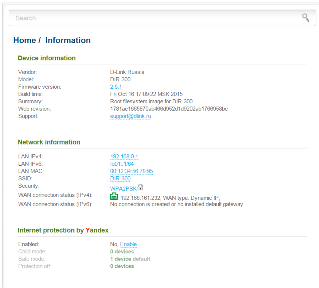
Figure 18. The general information page.
