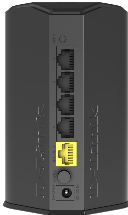
Figure 2. Back panel view.
